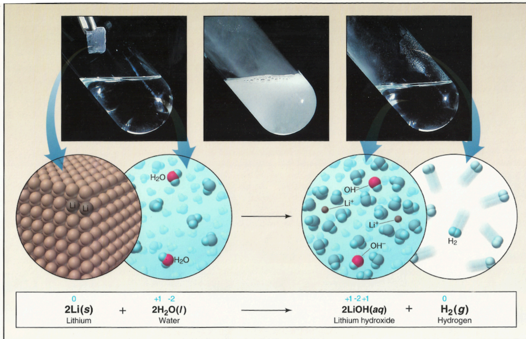
38 Three views of a single-displacement reaction Figure 4.17
