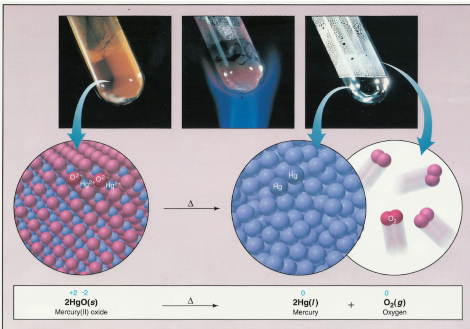
37 Three views of a decomposition reaction that forms elements Figure 4.16
