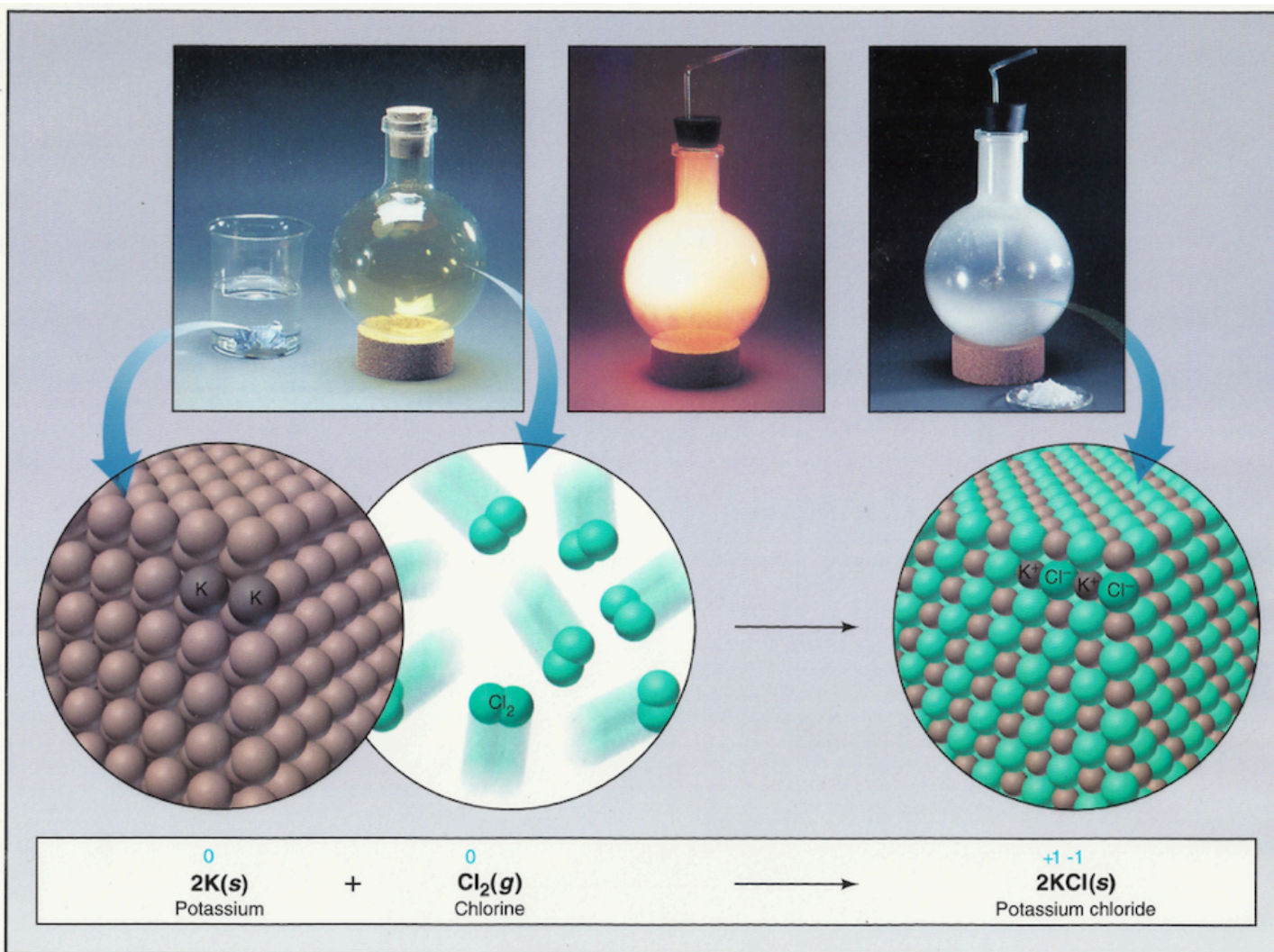
36 Three views of a combination reaction between elements Figure 4.15
